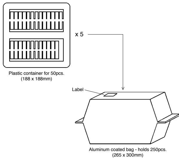
Figure 25 - Packing methodology
