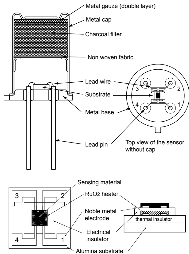
Figure 1 - Sensor structure
